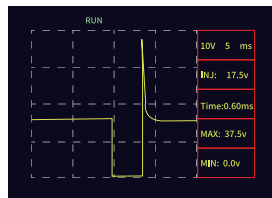
Fuel Injector test
